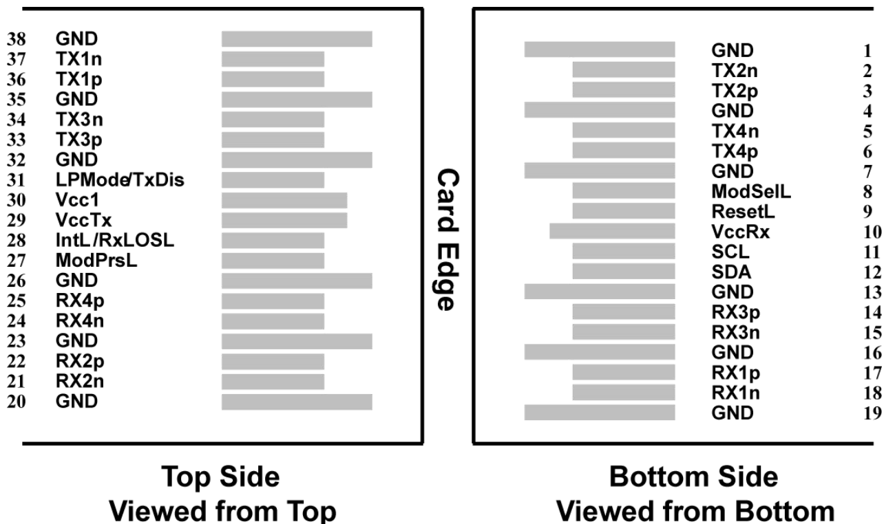
Figure 2 MSA compliant Connector
