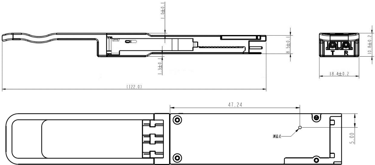
Figure 3 KWQE02-SW Mechanical Dimensions
