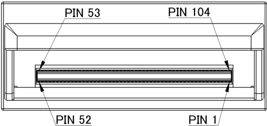
Figure 8. CFP2 Module Pad Layout
