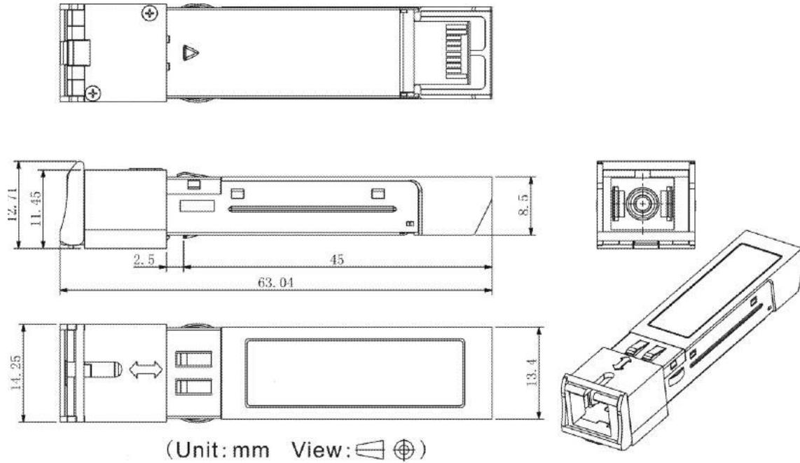
Figure 6. Mechanical Drawing
