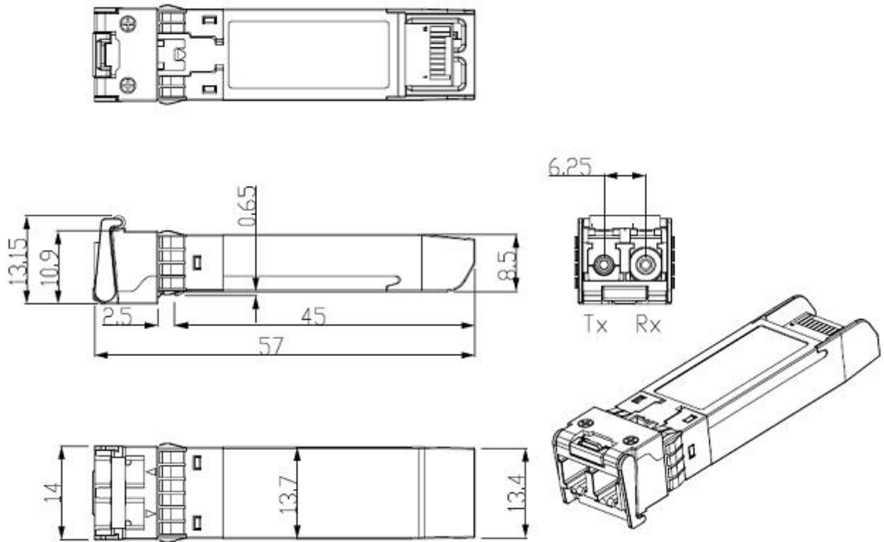
Mechanical Drawing
