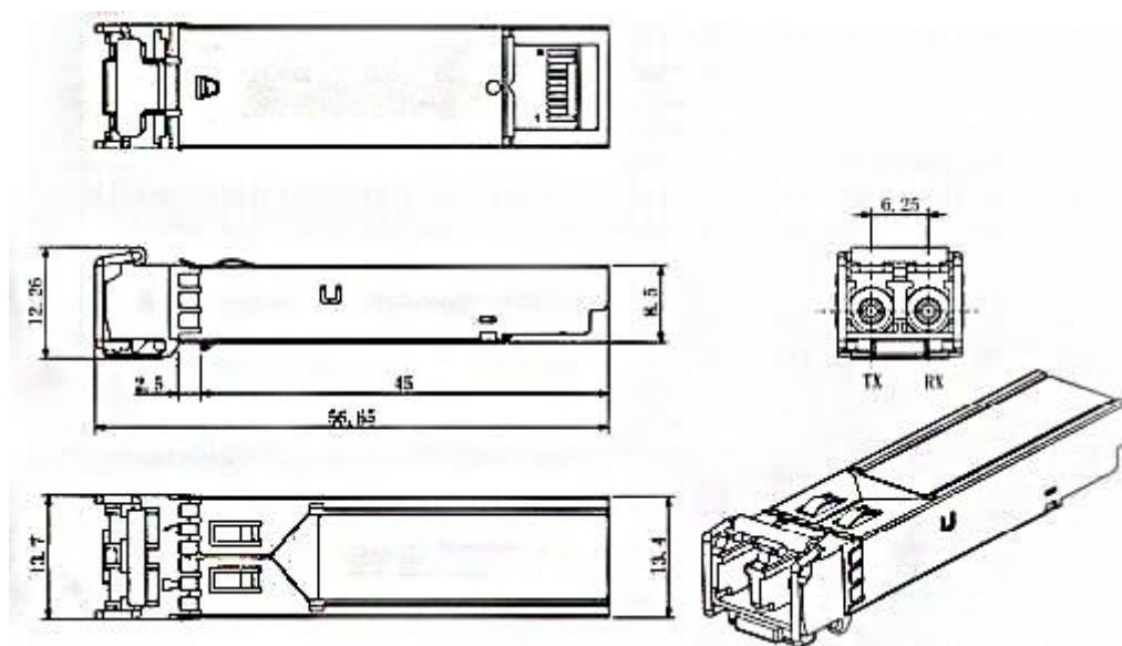
Mechanical Drawing
